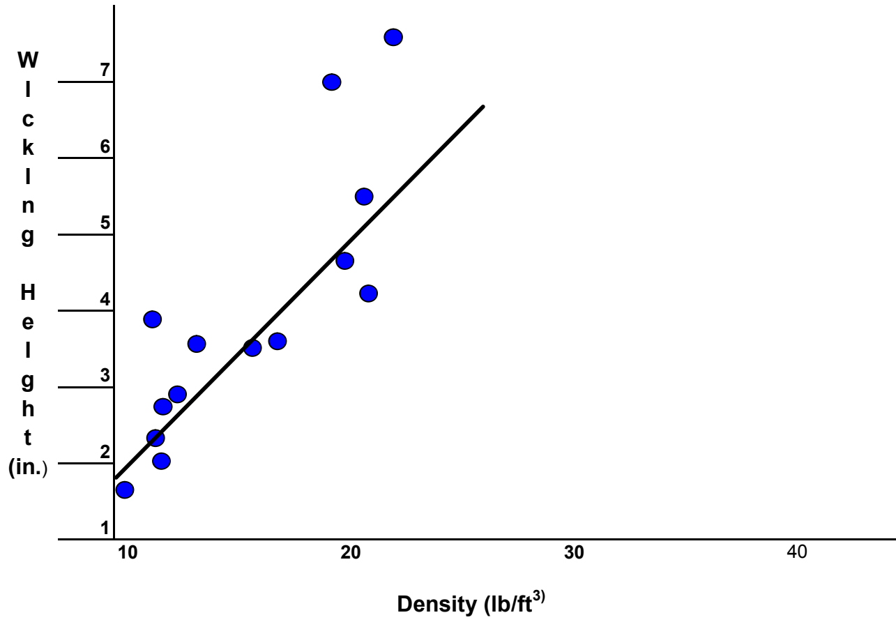
Figure 4 - Felt Density vs. Wicking Height
